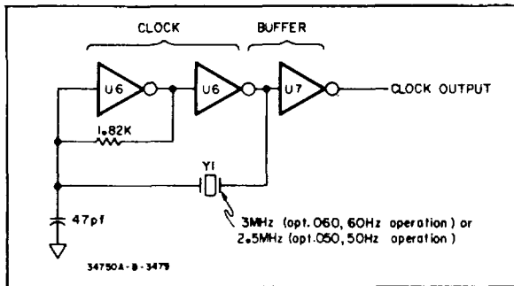
Figure 4-8. Data Clock.
