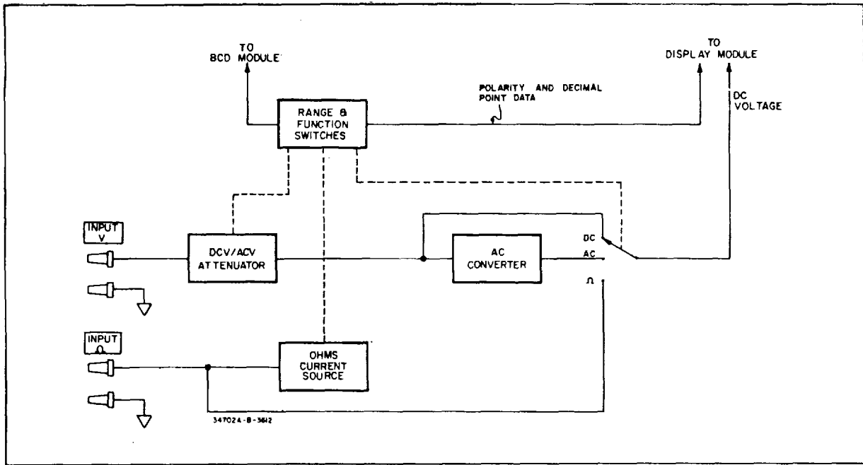
Figure 4-1. Block Diagram.
