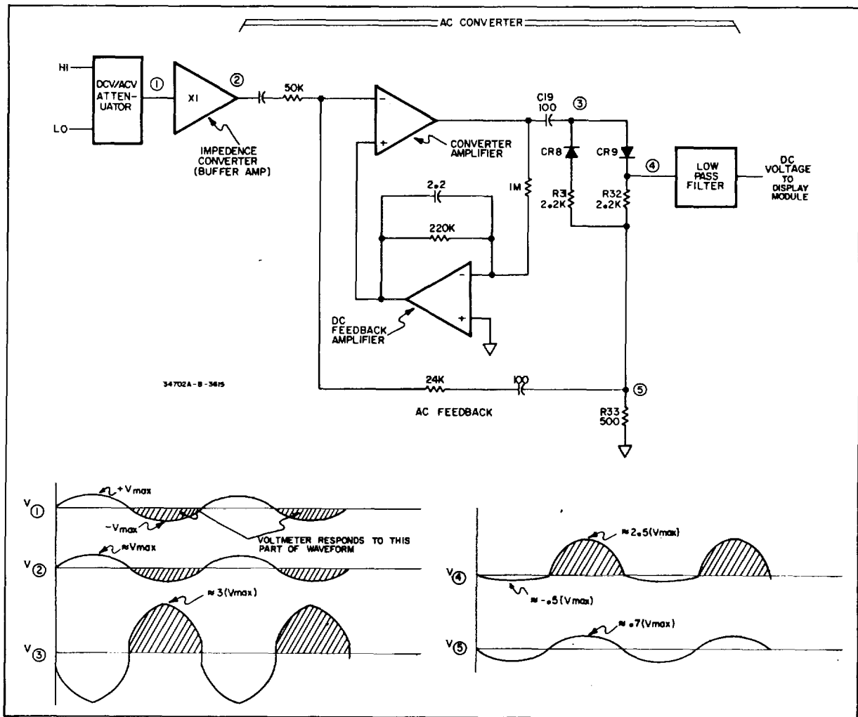
Figure 4-4. Ac/DC Converter.
