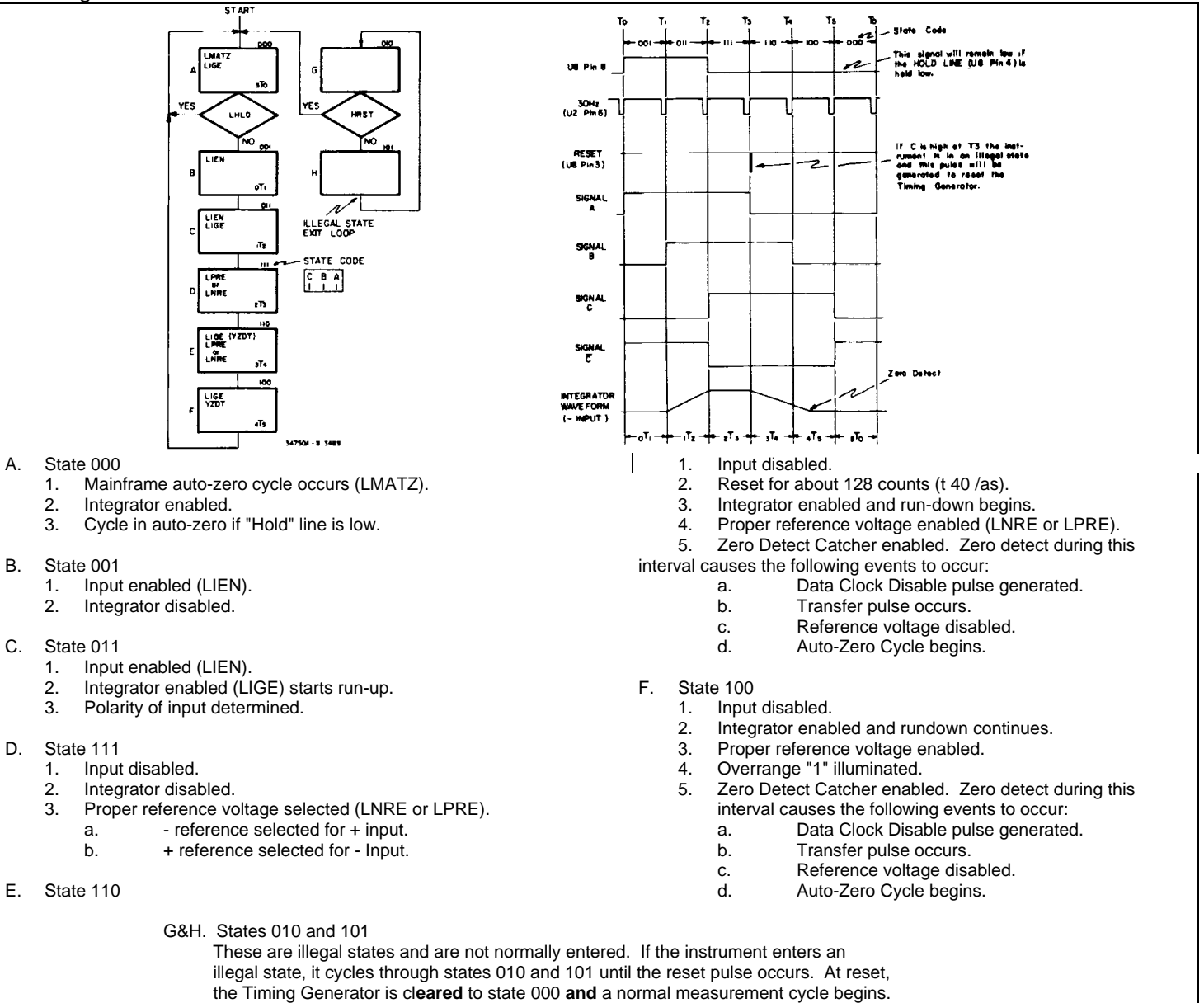
Figure 4-9. 34750A Flow Chart.
