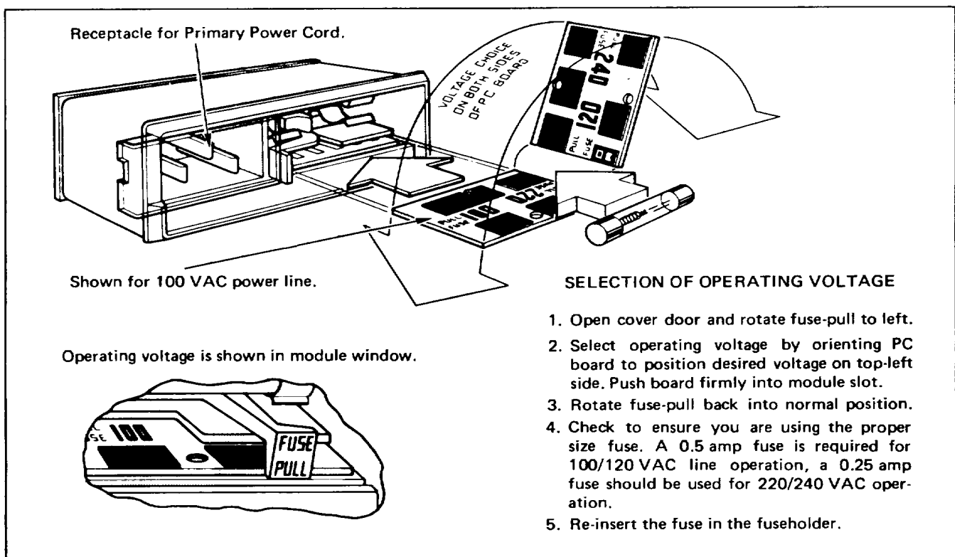
Figure 2-1. Voltage Selection.
