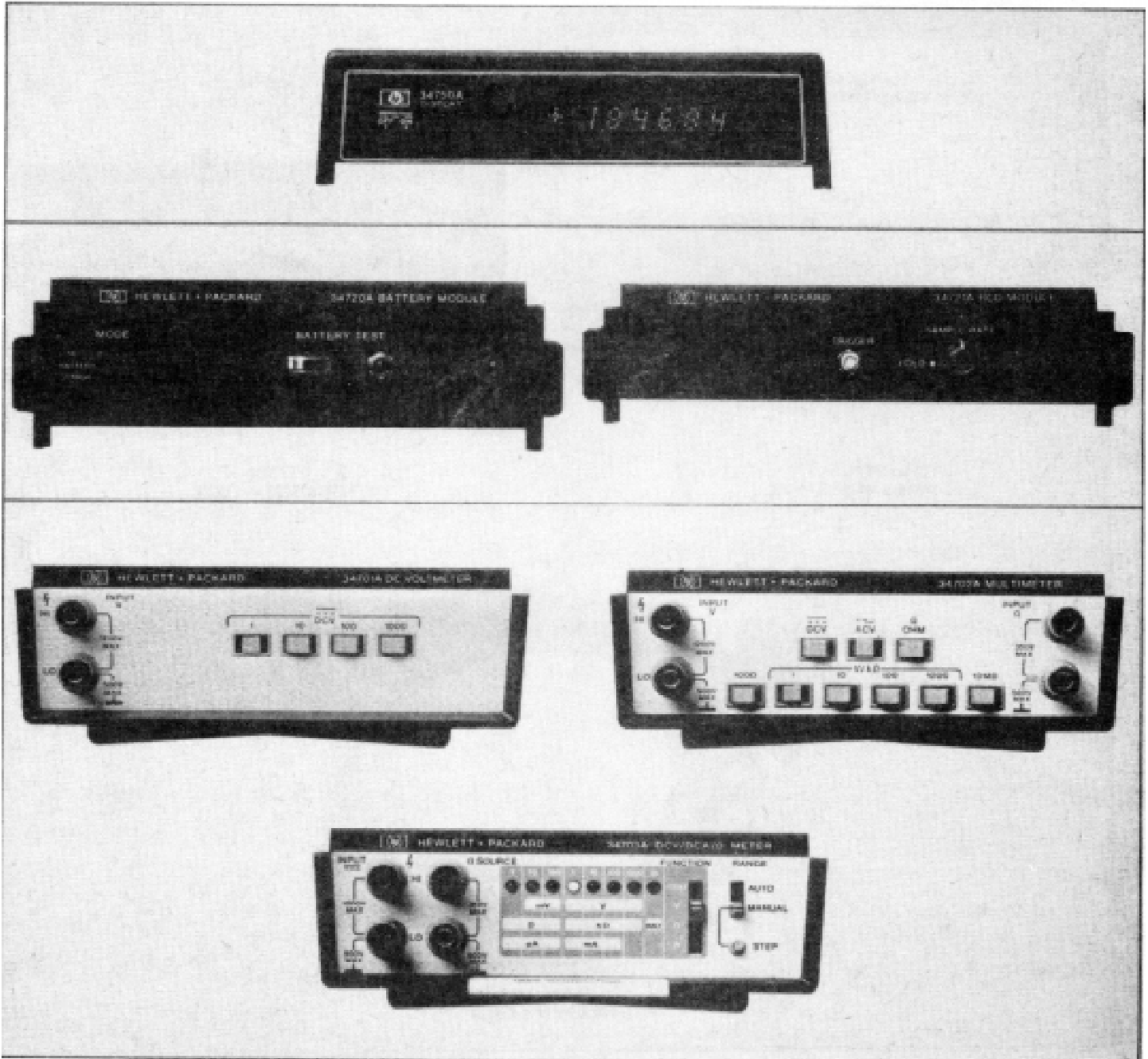
Figure 1-1. Plug-On Modules which can be used with the 34750A Display Module.
