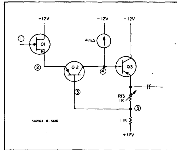
Figure 4-5. Impedance Converter.
