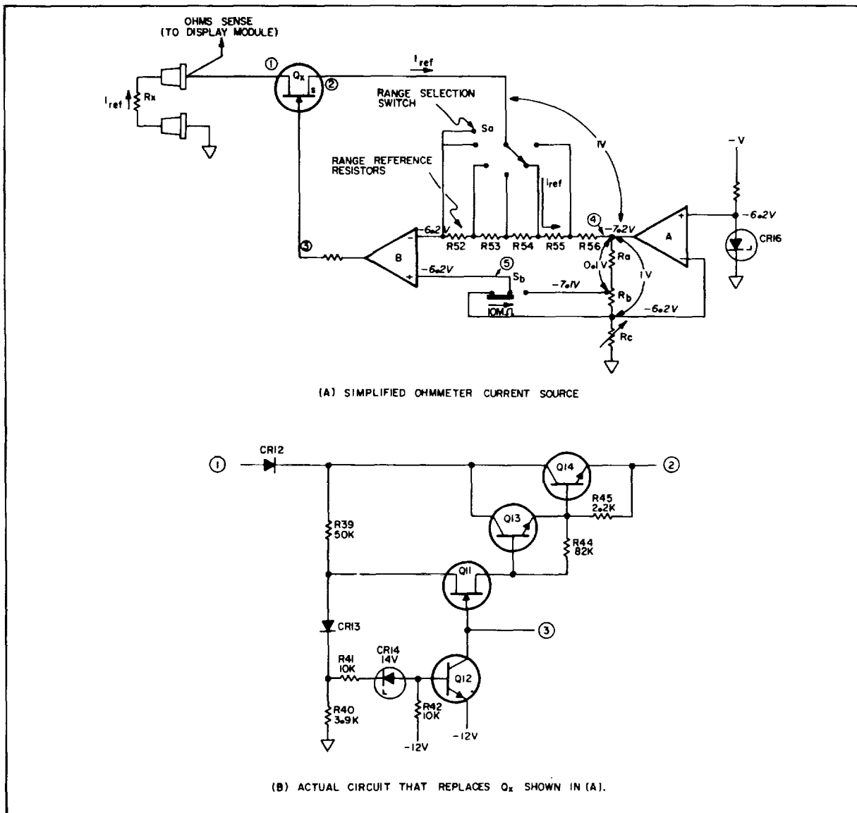
Figure 4-3. Ohms Converter.
