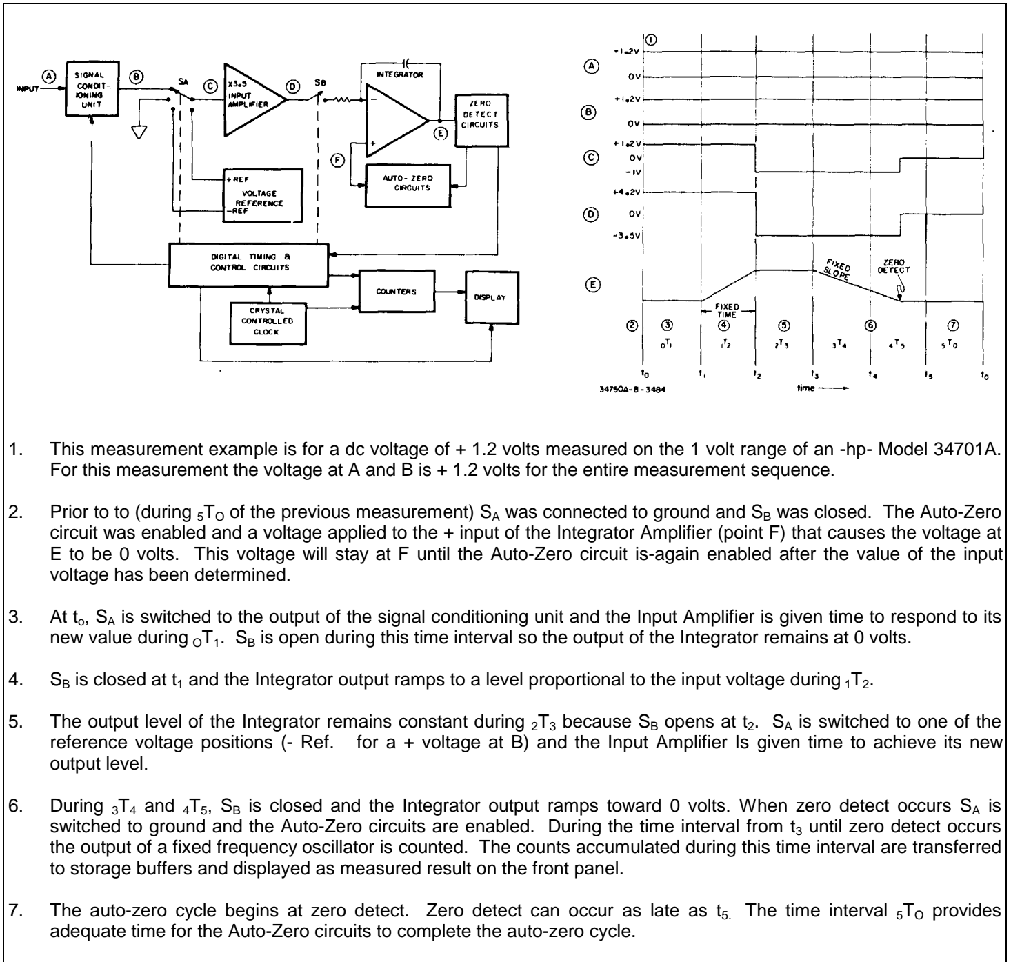
Figure 4-1. Basic Block Diagram of 34750A
